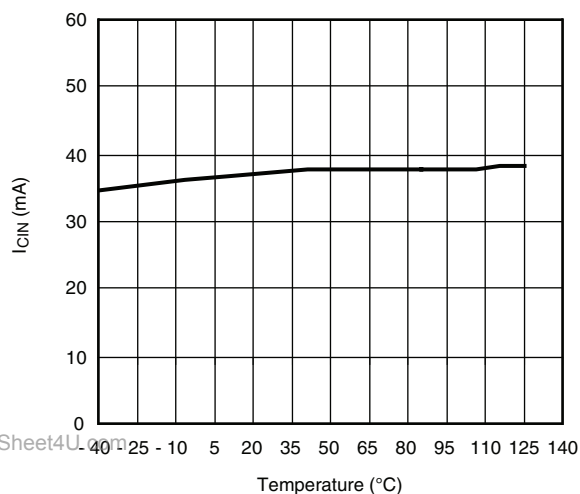
ICIN + IDRIV (mA) vs. Temperature at Frequency = 1 MHz D = 10\% , V_{CIN} = V_{DRV} = 5\text{ V}
